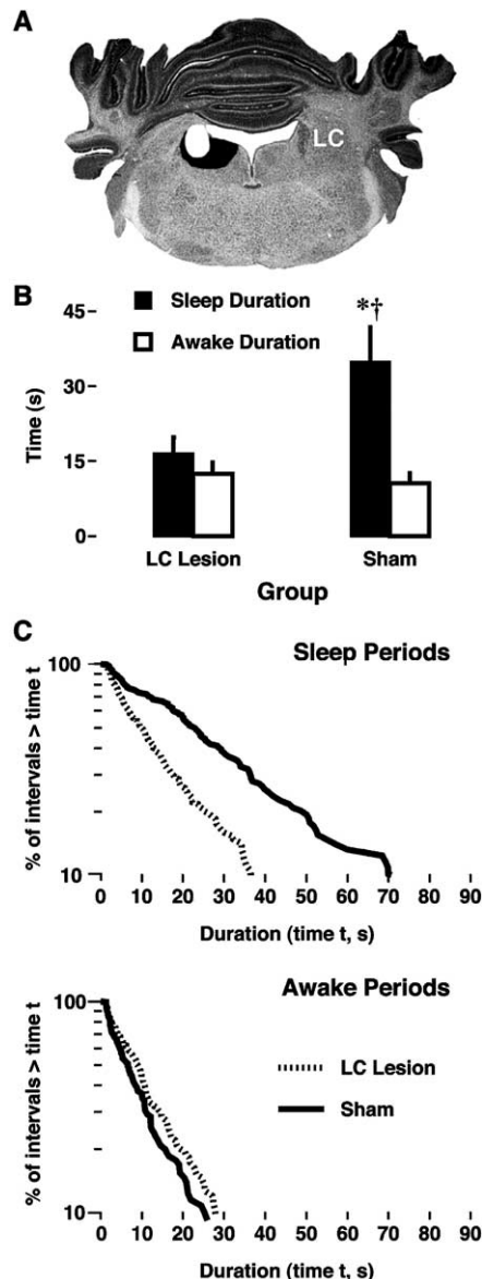
Fig. 4. Effect of bilateral LC lesions on nuchal EMG cyclicality in P8 rats. (A) Coronal section at the level of the LC in a P8 rat. The smallest lesion (white blob) and the largest lesion (black blob) are indicated. Lesions on the contralateral side (which are nearly identical) are not shown so that the LC, characterized by the densely staining vertical column of cells, can be visualized. (B) Mean sleep and awake durations for the pups with LC lesions and sham controls. * Significant difference from Awake Duration. † Significant difference from Sleep Duration in the lesion group. (C) Log-survivor plots of sleep periods (top) and awake periods (bottom) for the same subjects as in (B). Each plot is constructed from 114 data points (19 per subject).
